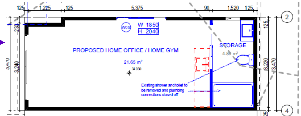
Existing outbuilding – Proposed floor plan
